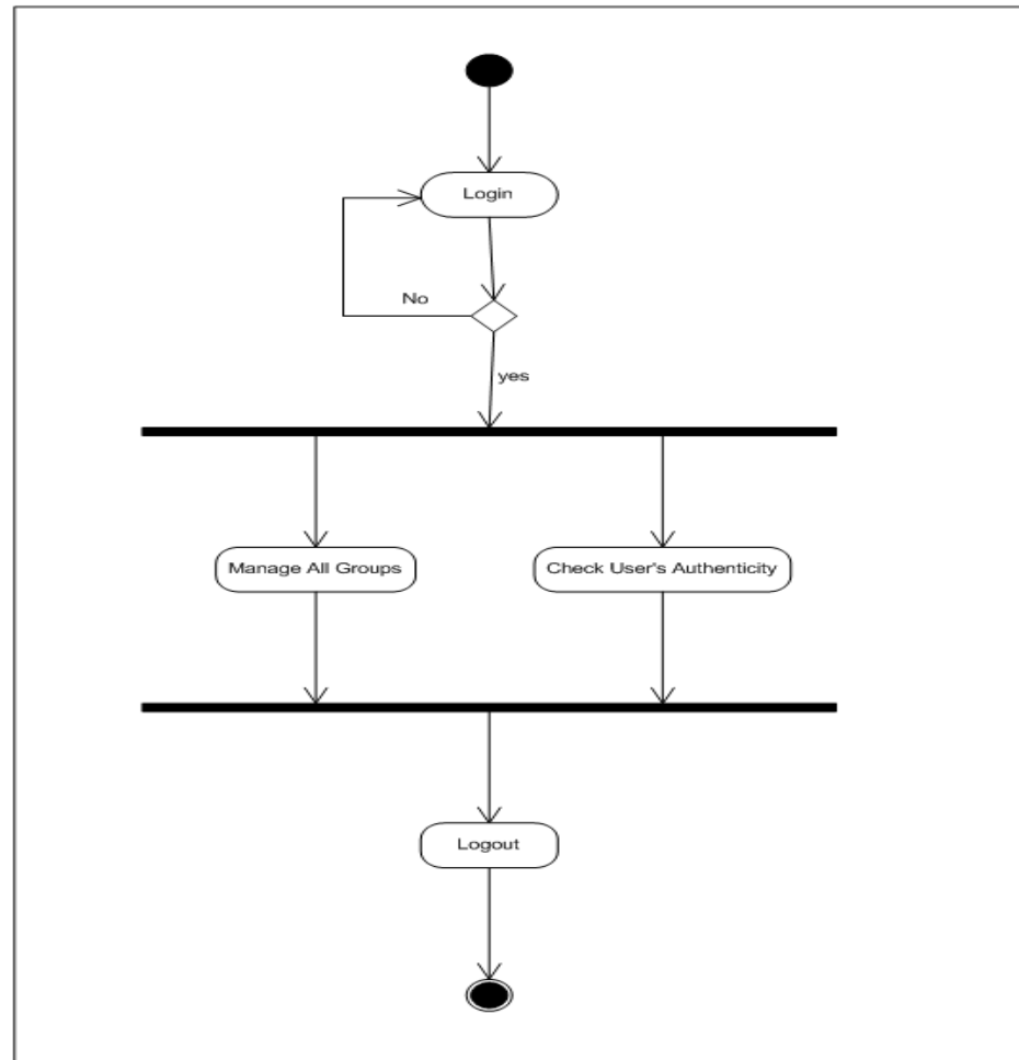
Activity Diagram
