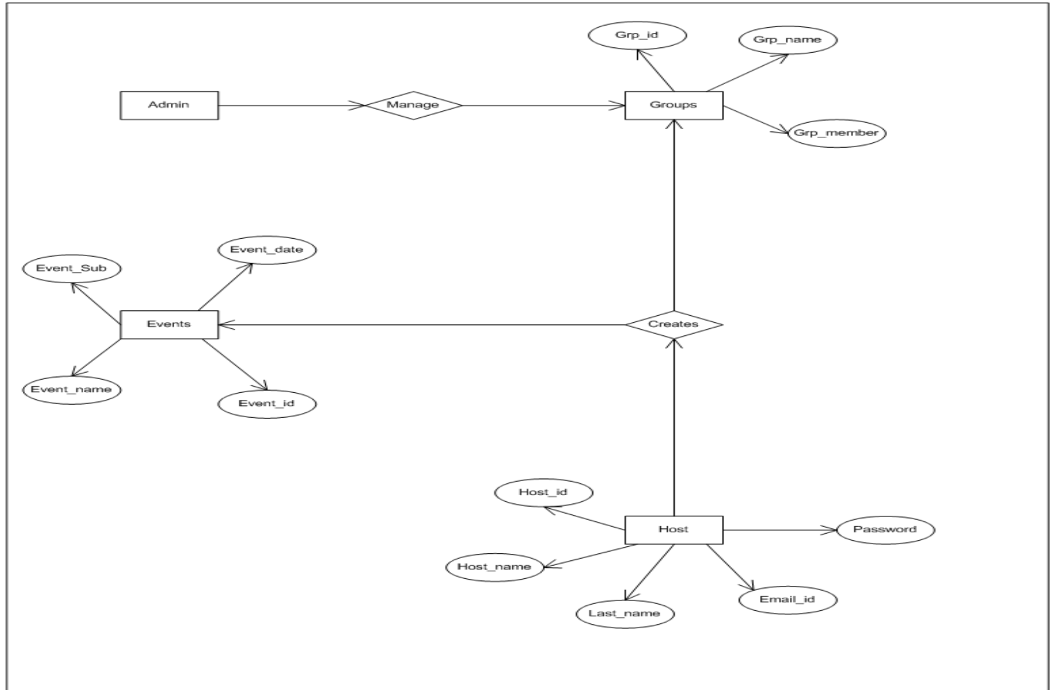
E-R Diagram
